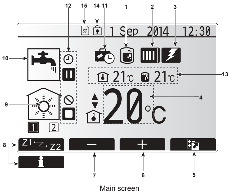
Main screen
